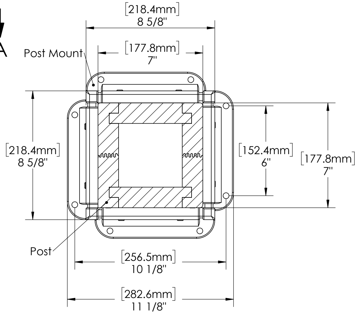
POST DETAIL
