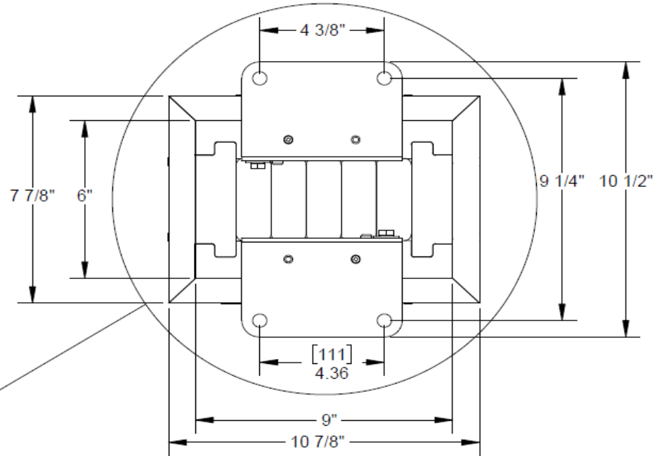
POST DETAIL
