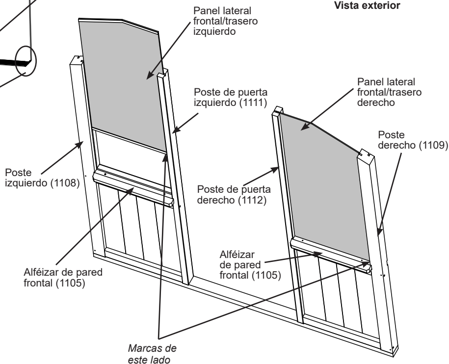
F2.14 Vista exterior
